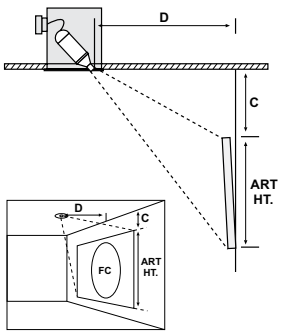
SLOTTED TRIM (STANDARD)
